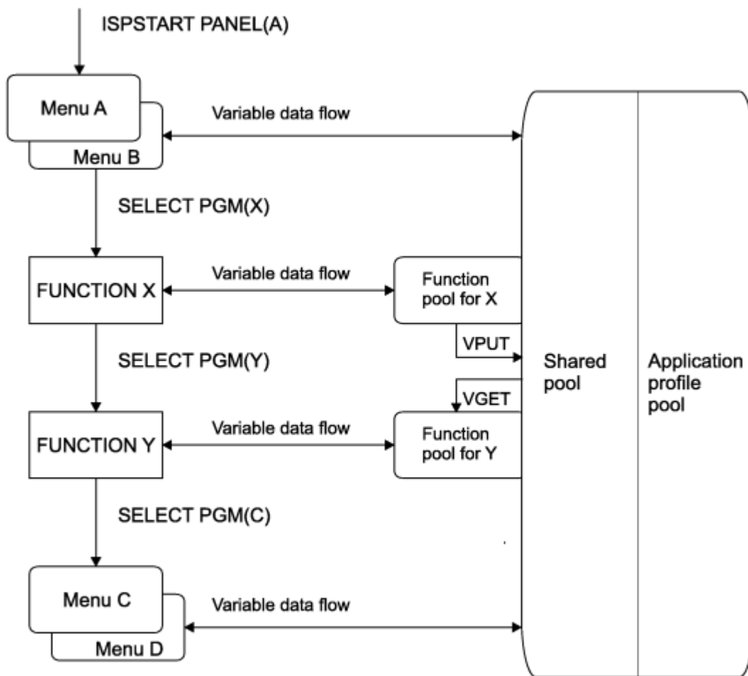
Figure 21. Control and data flow in a dialog
